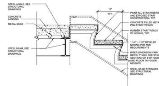
1 LANDING AND RISER DETAIL 1 1/2" x 1 1/2"
