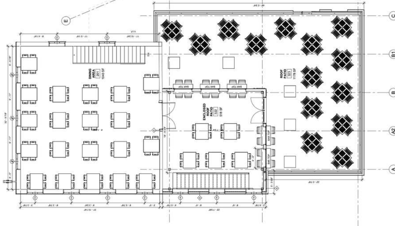
1 SECOND FLOOR 1/8" = 1'-0"
